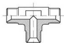
RACCORDO 3 VIE M+M+M BSP 60°
