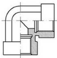
GOMITO F - F BSP
