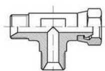
RACCORDO 3 VIE M+M+F.GIR. BSP 60°
