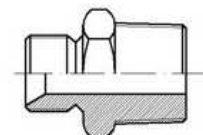
NIPPLLO RID. M - M CIL. BSP 60°- CONICO
